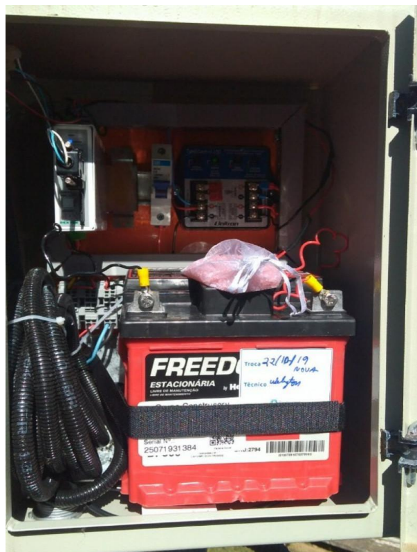
Interior do Painel
